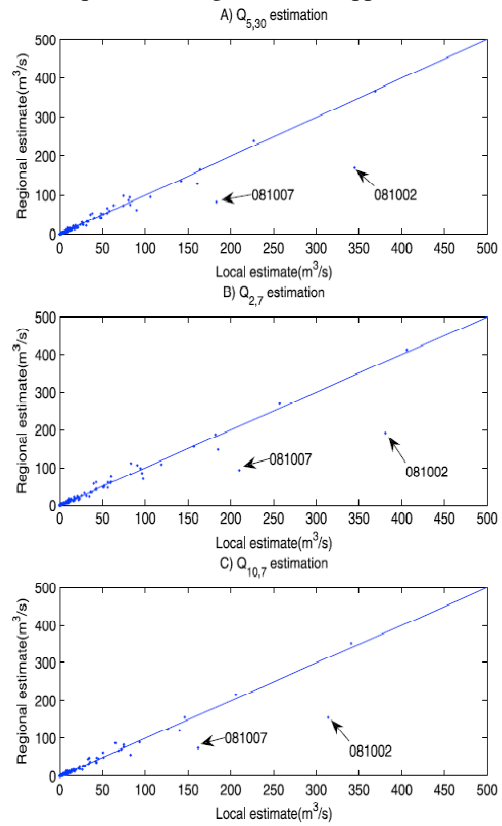
9. Jackknife estimation of the winter low-flow quantiles using the regression approach
