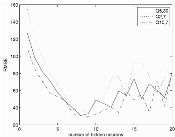
Fig. 2. RMSE of summer low-flow estimation using single ANN models with the number of hidden neurons increased from 1 to 20
