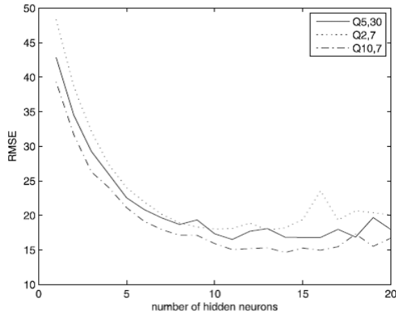
Fig. 3. RMSE of winter low-flow estimation using single ANN models with the number of hidden neurons increased from 1 to 20
