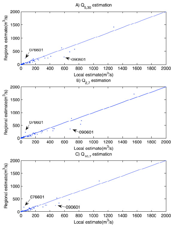
Fig. 6. Jackknife estimation of the summer low-flow quantiles using the regression approach
