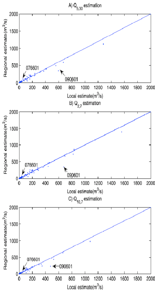
Fig. 4. Jackknife estimation of the summer low-flow quantiles using the SANN approach
