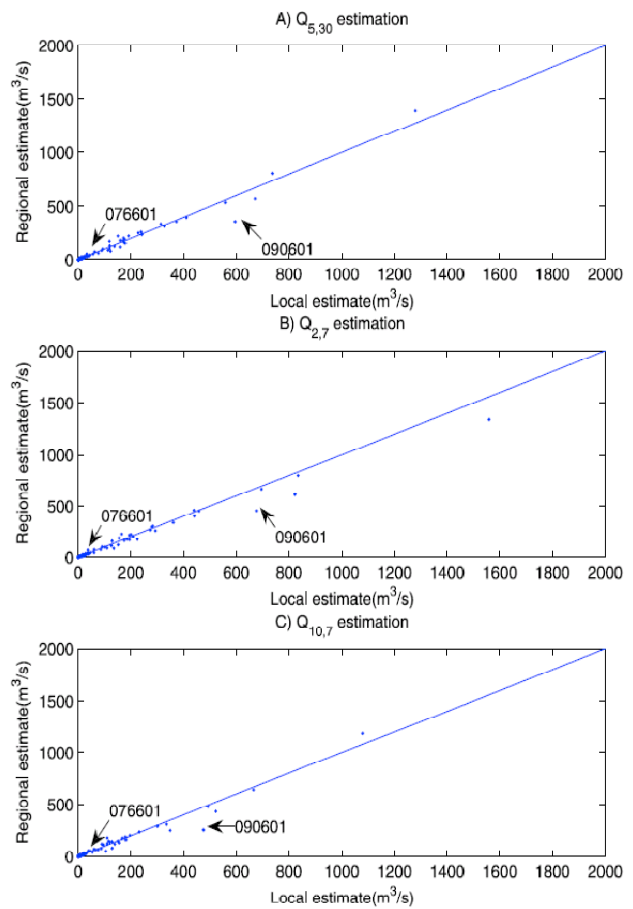
Fig. 5. Jackknife estimation of the summer low-flow quantiles using the EANN approach
