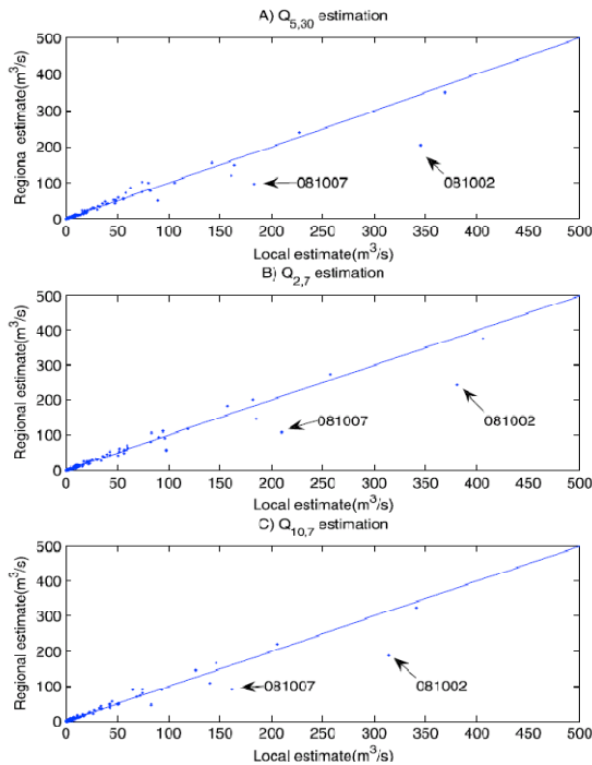
Fig. 8. Jackknife estimation of the winter low-flow quantiles using the EANN approach
