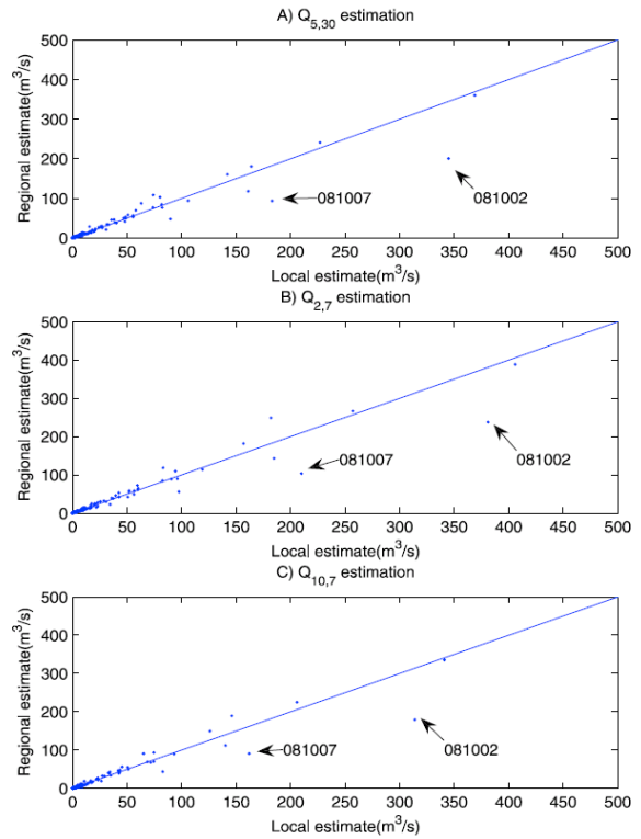
Fig. 7. Jackknife estimation of the winter low-flow quantiles using the SANN approach.
