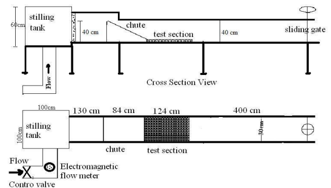
Fig. 2. Experimental facilities
