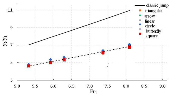
Fig. 5. y_2/y_1 versus F_r for different layouts of the SLC elements
