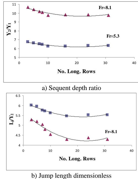
Fig. 8. y_2/y_1 and L_j/y_2 versus number of SLC elements longitudinal rows
