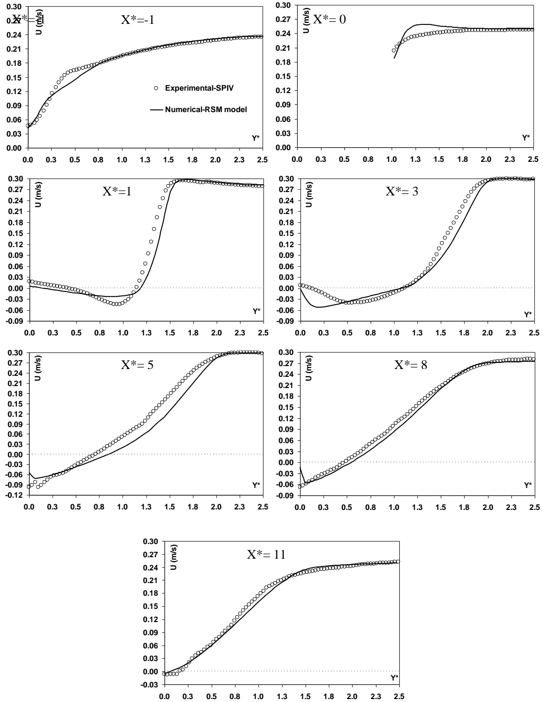
Fig. 5. Comparison of the transverse velocity profiles between SPIV measurements and numerical simulation using RSM turbulence model
