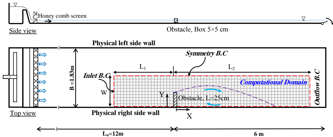
Fig. 2. Geometrical specifications of the test case (Safarzadeh and Salehi, 2013). The area denoted by red dashed lines shows the computational domain in the present numerical simulation.
