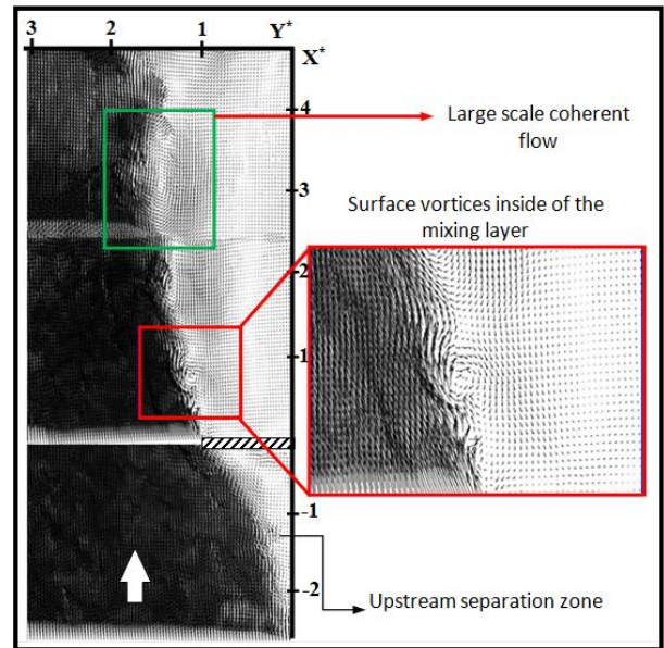
Fig.1. Temporal flow structure generated by side obstacle and obtained by SPIV Measurement (Safarzadeh and Salehi, 2013)
