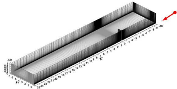
Fig. 3. Computational mesh for W=7.3L case
