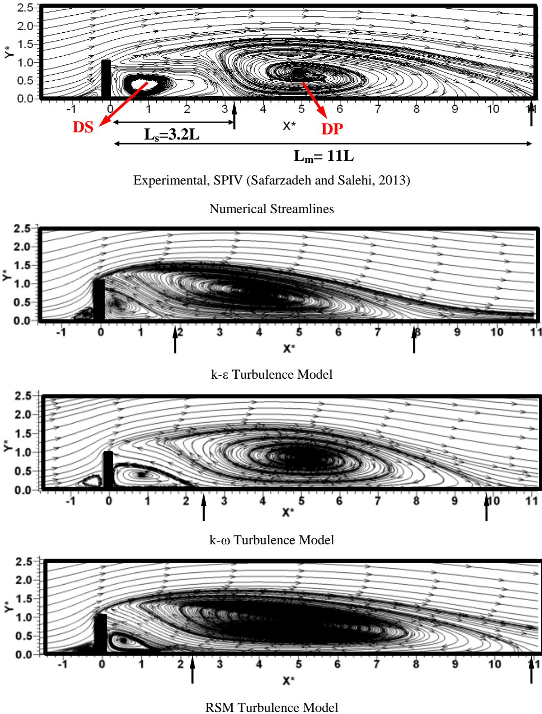
Fig. 4. Comparison of the stream line at water surface plane between SIV measurement (Safarzadeh and Salehi, 2013) and numerical result with various turbulence models
