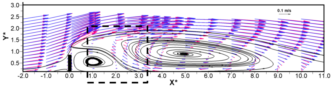
Fig.7. Comparison of the measured (Red) and RSM simulated (Blue) velocity vectors
