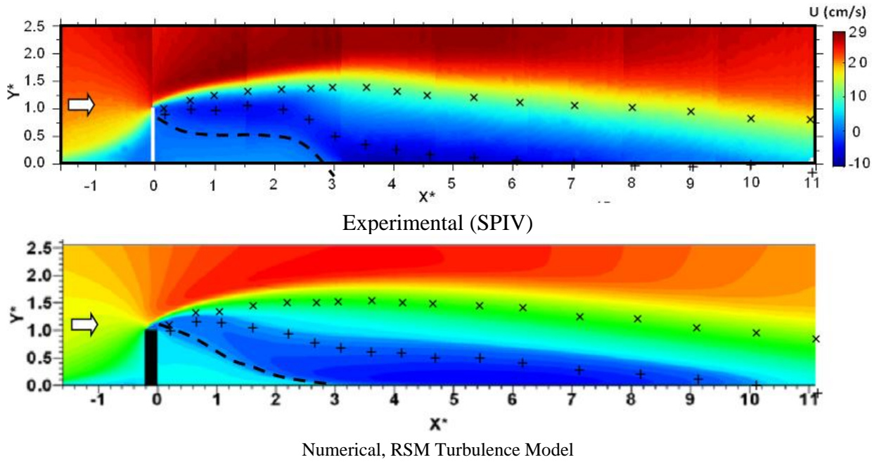
Fig. 6. Comparison of the stream wise velocity contours between SPIV measurements and numerical simulation using RSM turbulence model. “+” and “x” symbols denote inner and outer boundaries of the mixing layer, respectively
